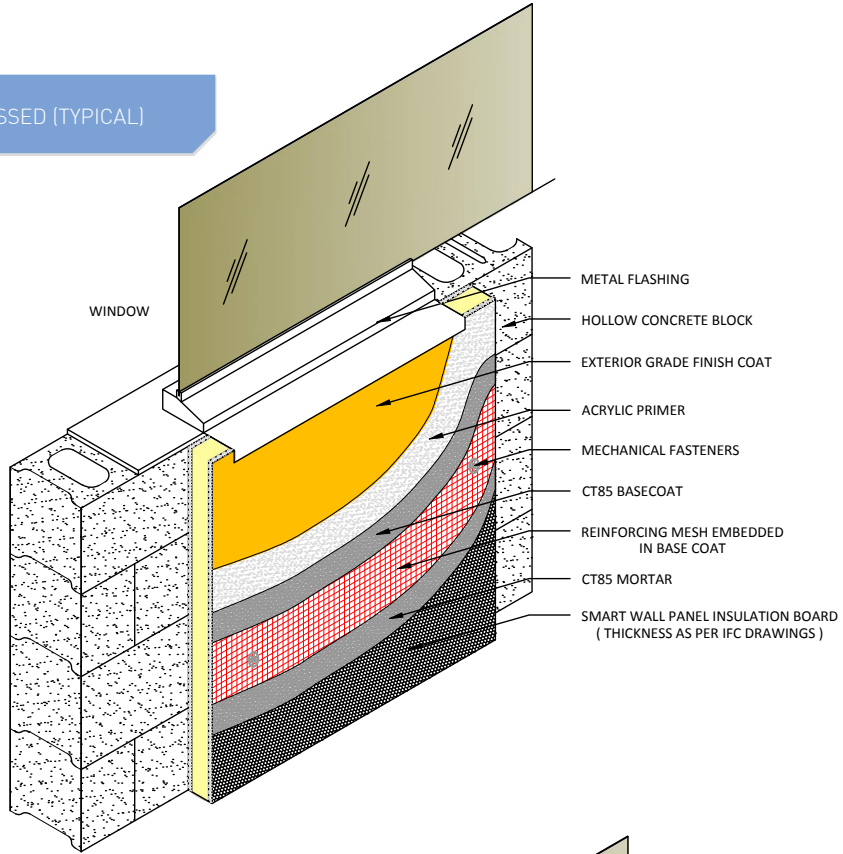
WINDOW SILL FLUSHED (TYPICAL)
