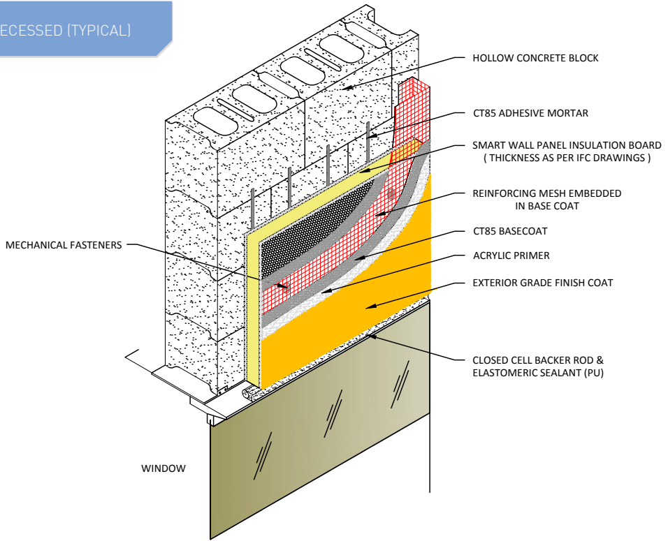
WINDOW HEAD FLUSHED (TYPICAL)
